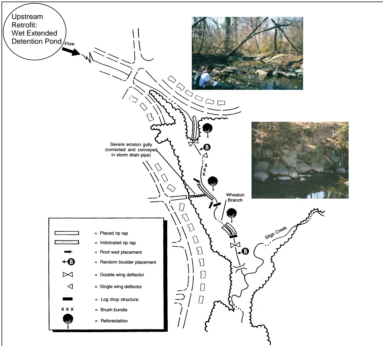
Figure 21: Example of Comprehensive Stream Restoration Approach
