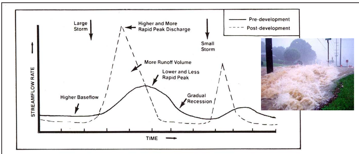
Figure 13: Comparison of Urban and Rural Hydrographs
