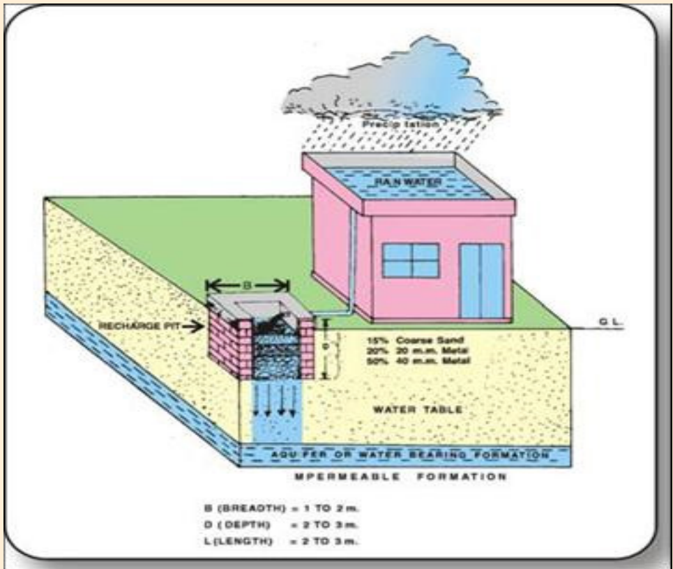
Figure (4.1) Rainwater harvesting recharge pit [14]
