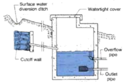
Figure 2: Cut-away view of a concentrated spring (Jennings,1996)
